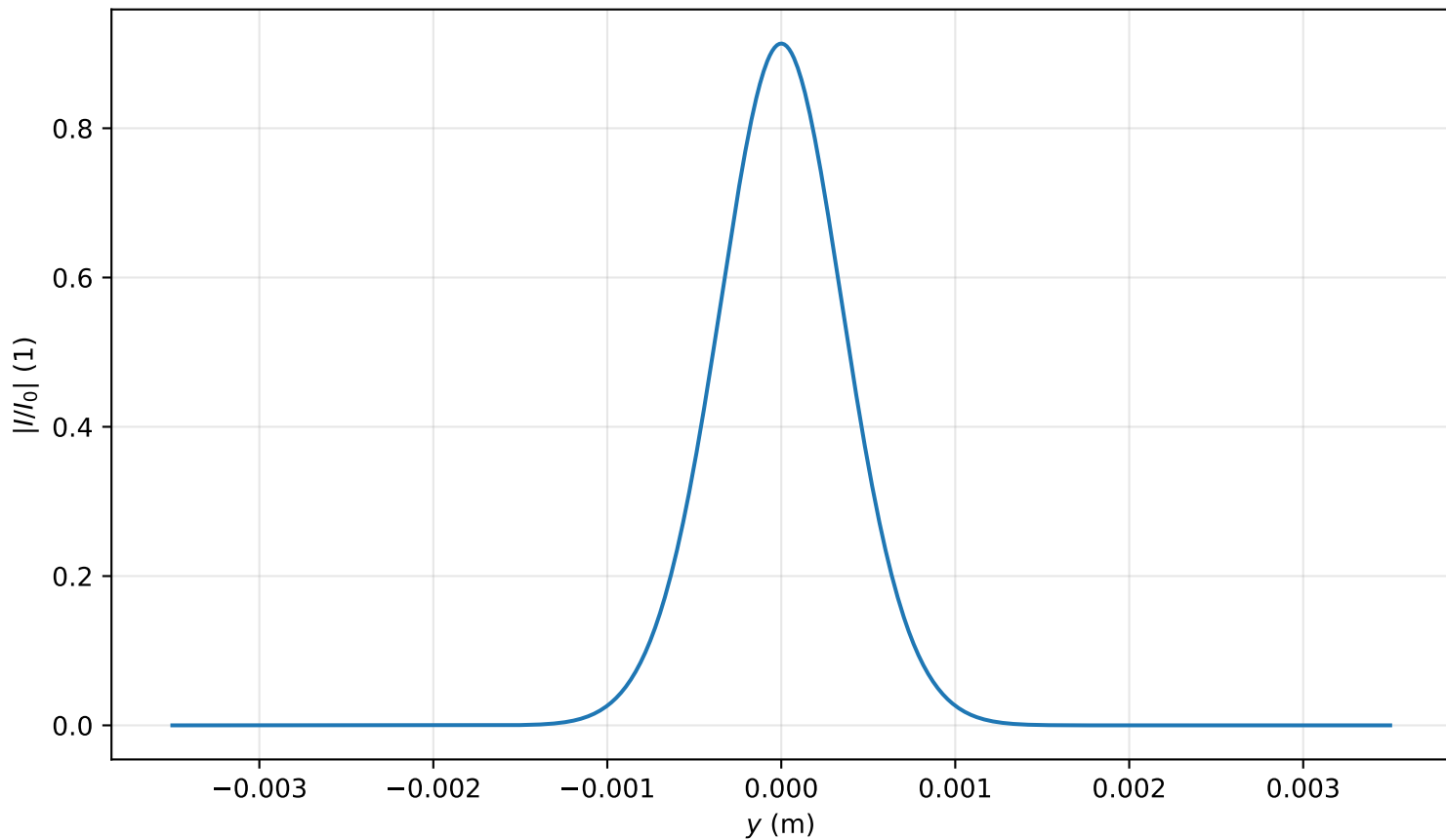
Intensity profile I(x=0, y, z=0.876)/I_0 , P_{in}=0.2P_{cr} , artificial time
